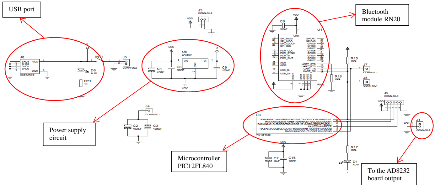
Fig.5 The digitalization and transmission block
