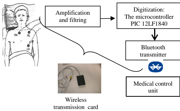
Fig. 1 Block diagram of the data acquisition system.
