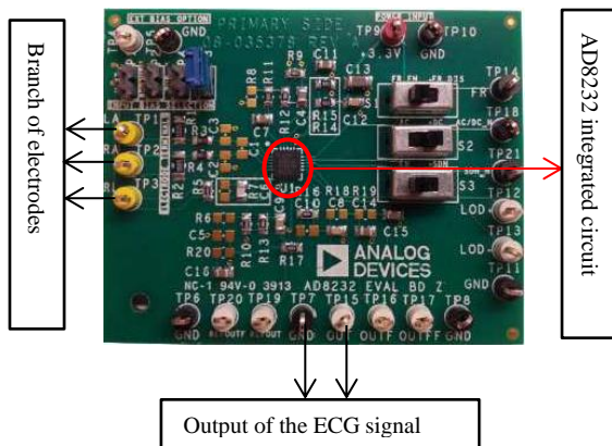
Fig. 2 The AD8232-EVALZ printed circuit board
