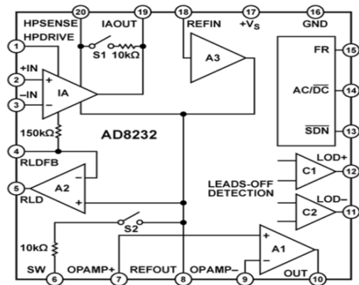
Fig. 3 Block diagram of AD8232
